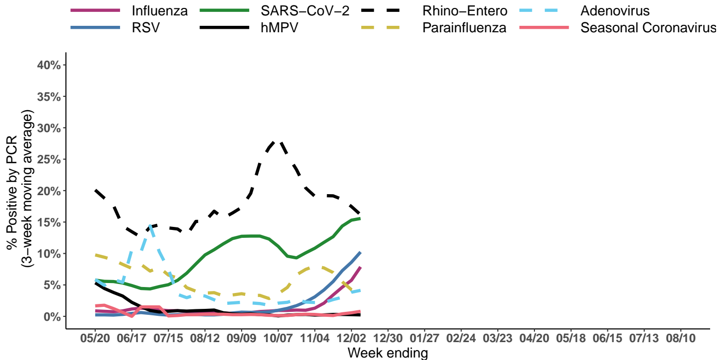
Number and percent positivity of respiratory viruses tested by PCR, NREVSS Week 49, Ending on December 09, 2023
